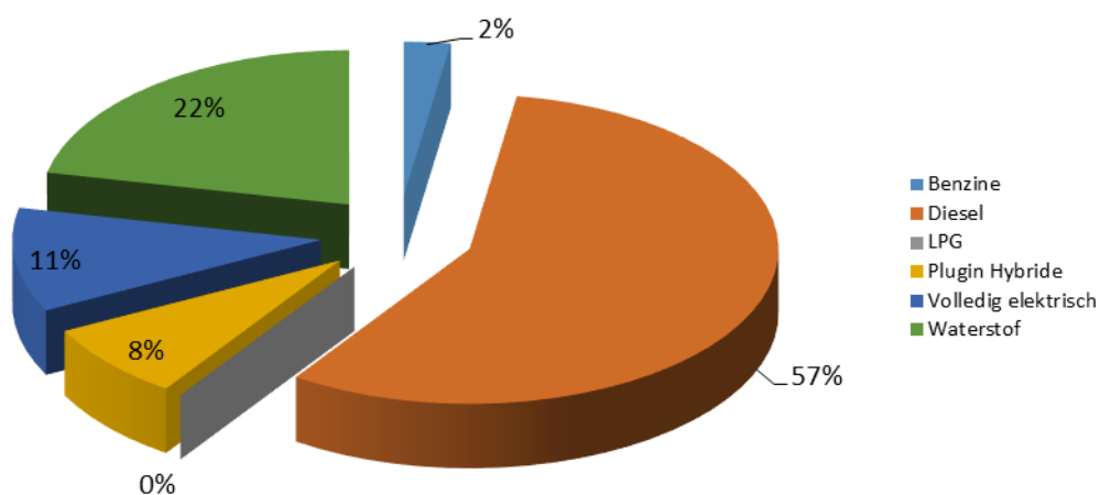
Emissies personenauto's
